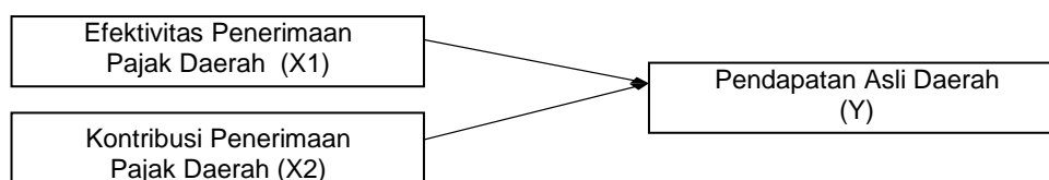
Gambar 1. Model Penelitian
